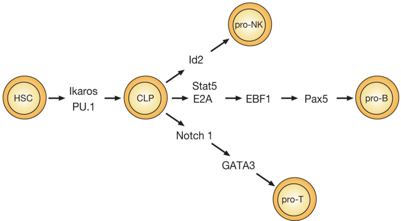
Figure 4. Transcriptional Control of Early Lymphopoiesis
